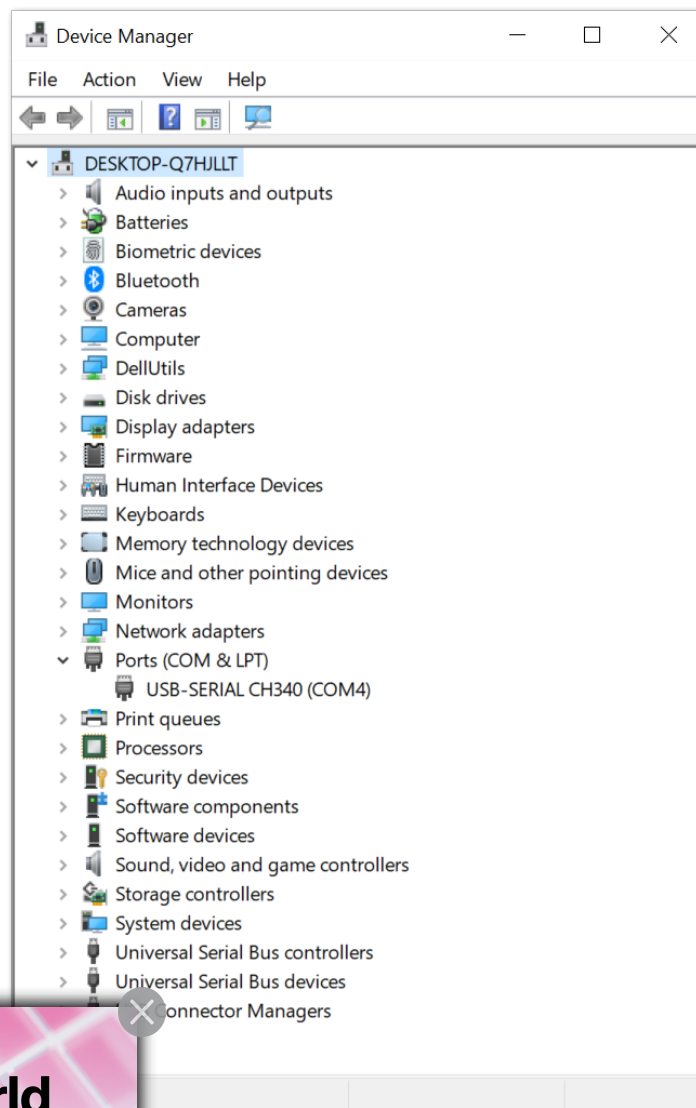
Figure 3: Device Manager
