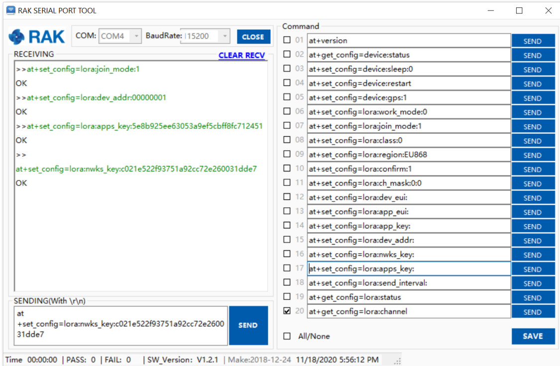
Figure 27: Configuring the WisNode Button 4K in ABP mode
