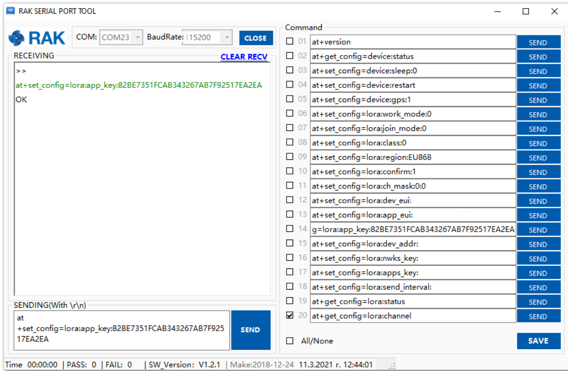
Figure 47: Setting up the RAK7201 WisNode Button 4K OTAA parameters
