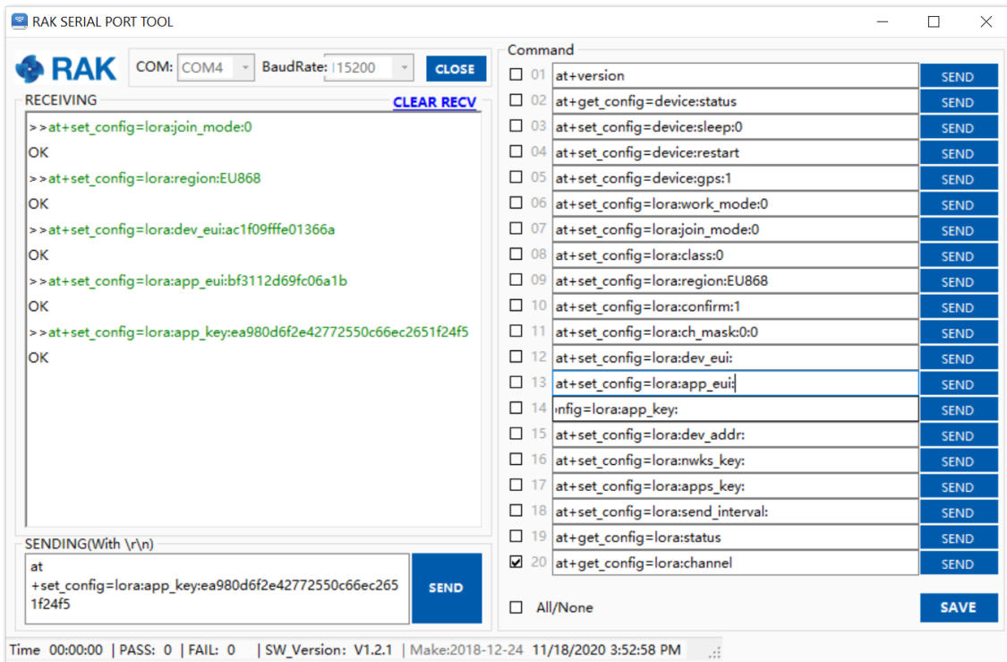
Figure 21: Configuring the RAK WisNode Button 4k in OTAA mode
