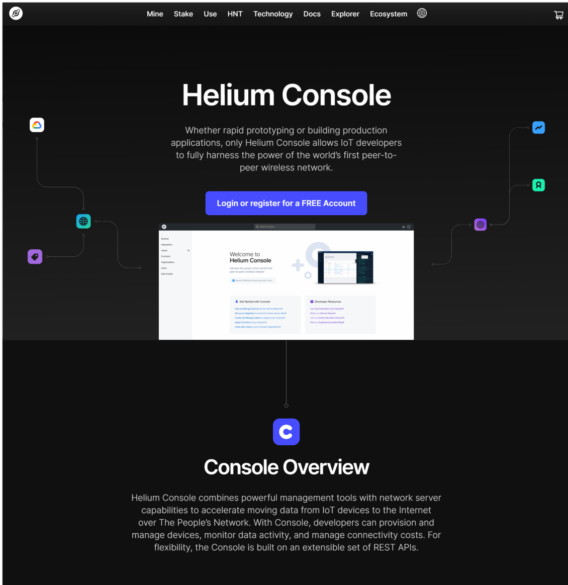
Figure 7: Helium console
