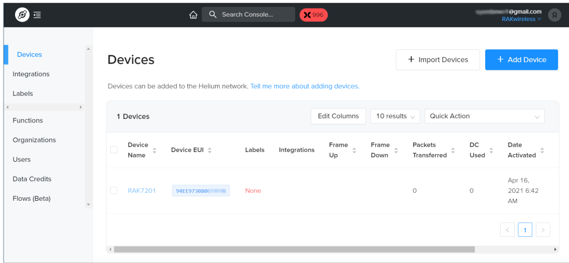
Figure 11: Helium devices
