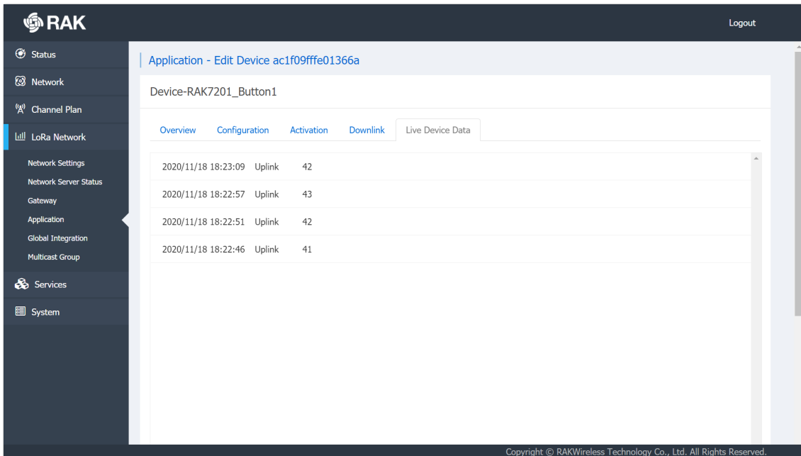
Figure 30: Received data
