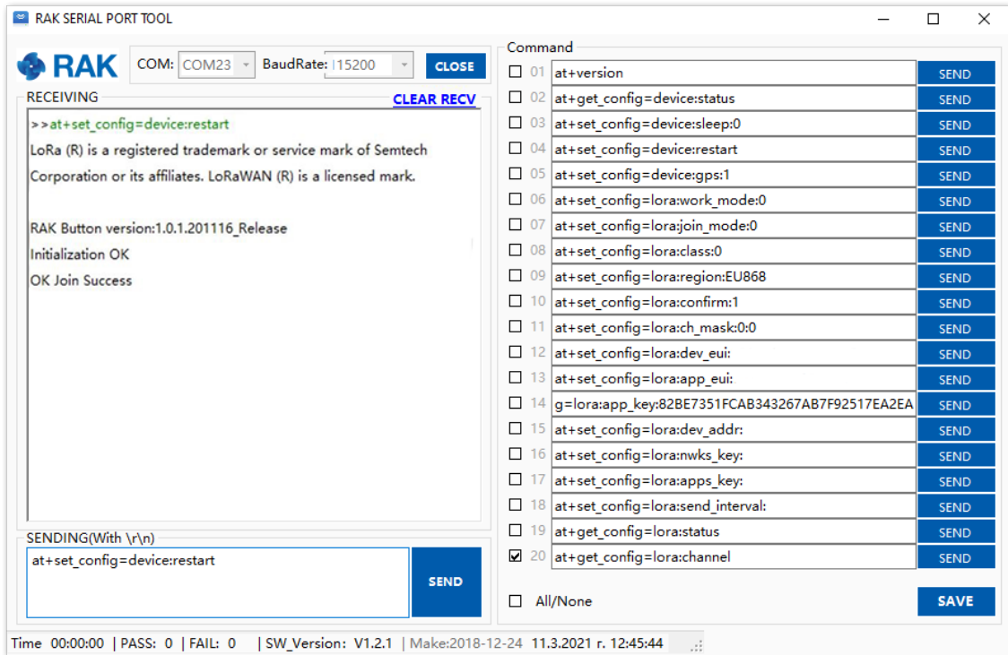
Figure 48: Join confirmation
