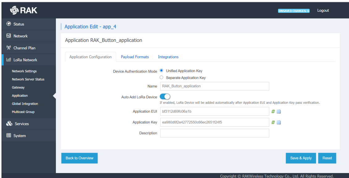
Figure 16: Application settings
