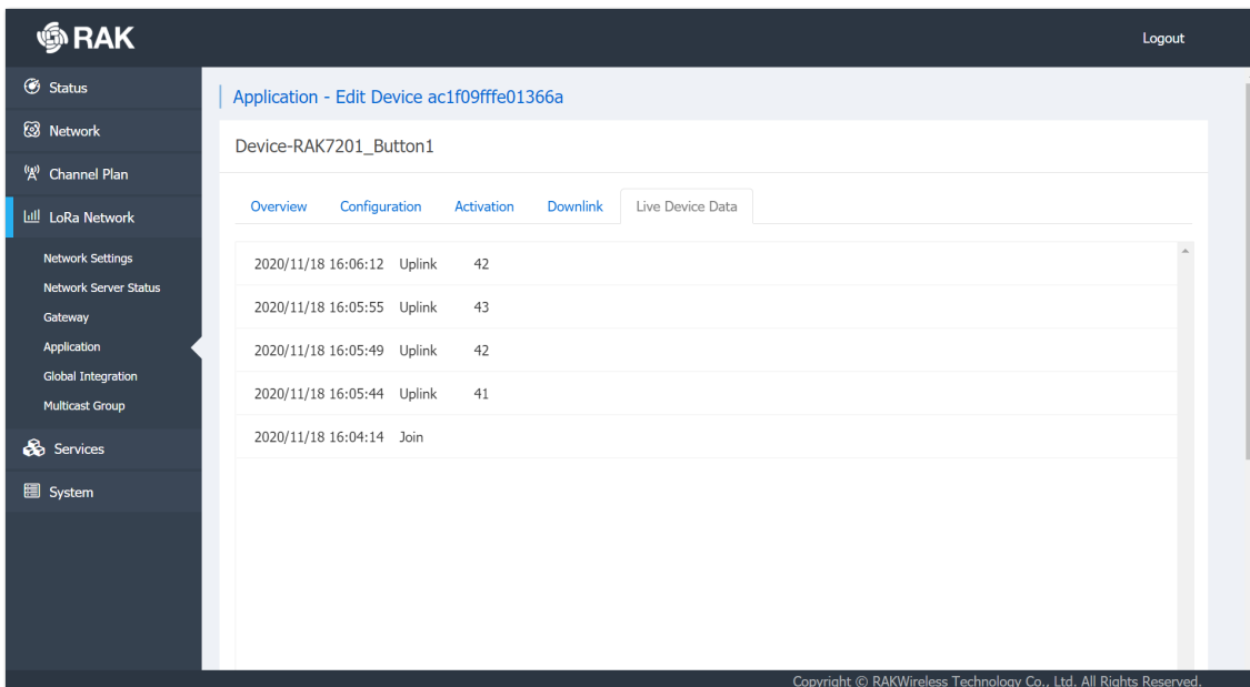
Figure 24: Received data
