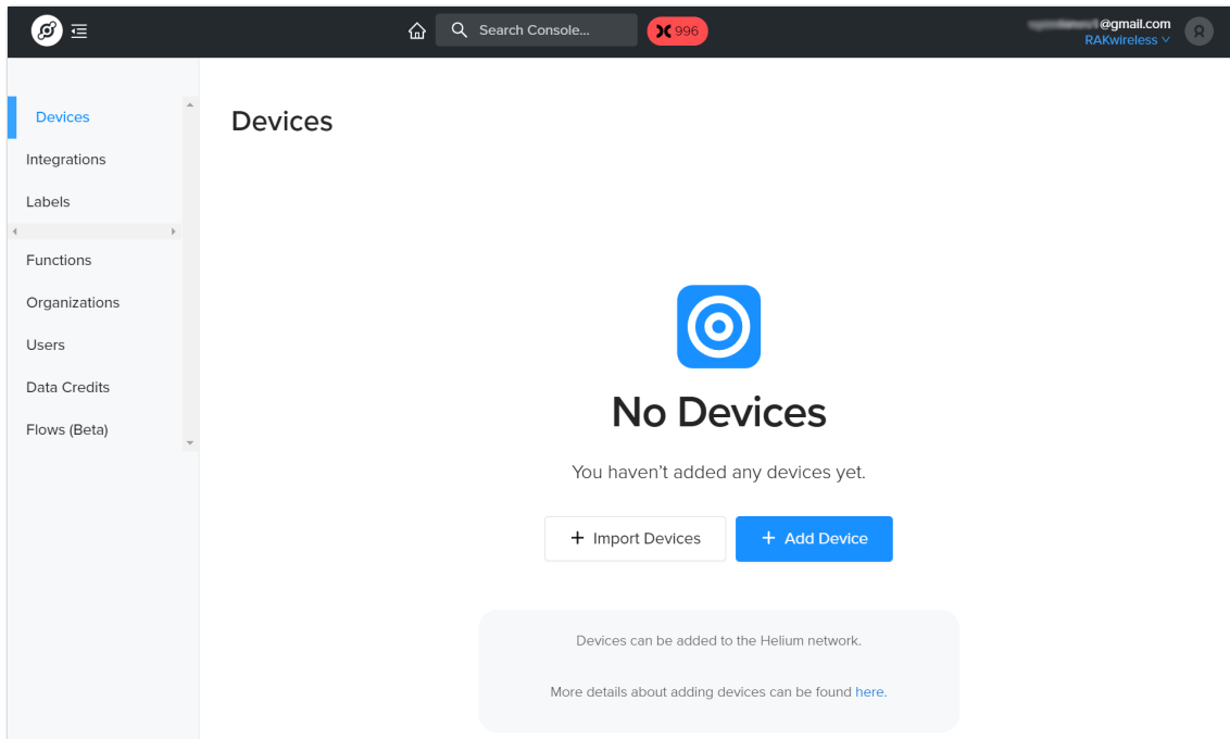
Figure 9: Helium devices
