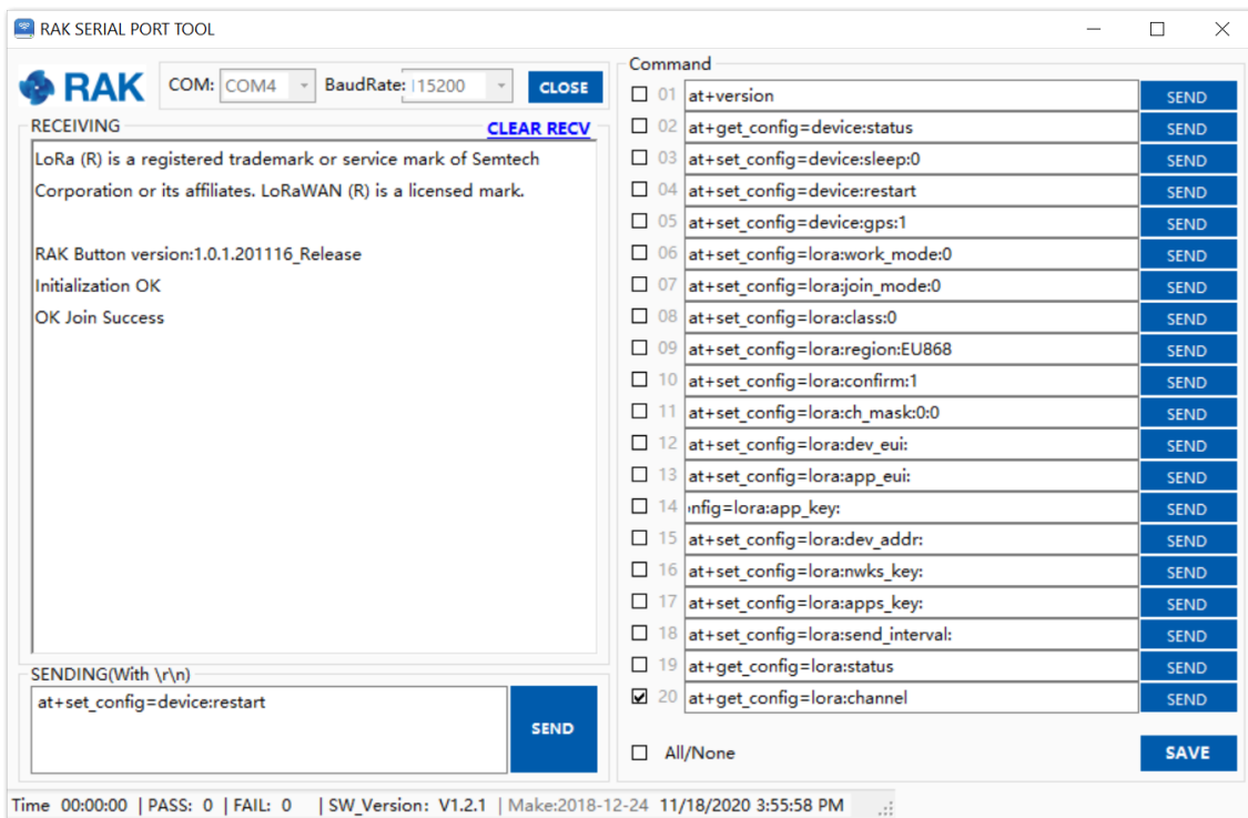
Figure 22: The device has restarted and connected to the LoRaWAN Network
